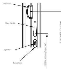
14 - Locking Slave Handle Layout Detail
