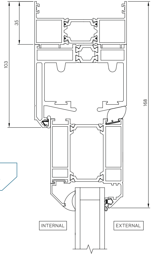
24c Bi-Fold Frame Extender With Trickle Vent
