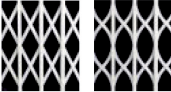
Standard 'X' lattice
