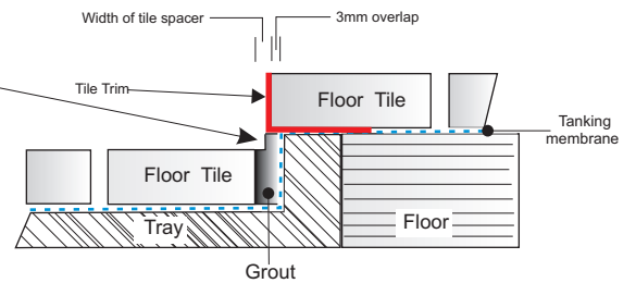
Section Through
