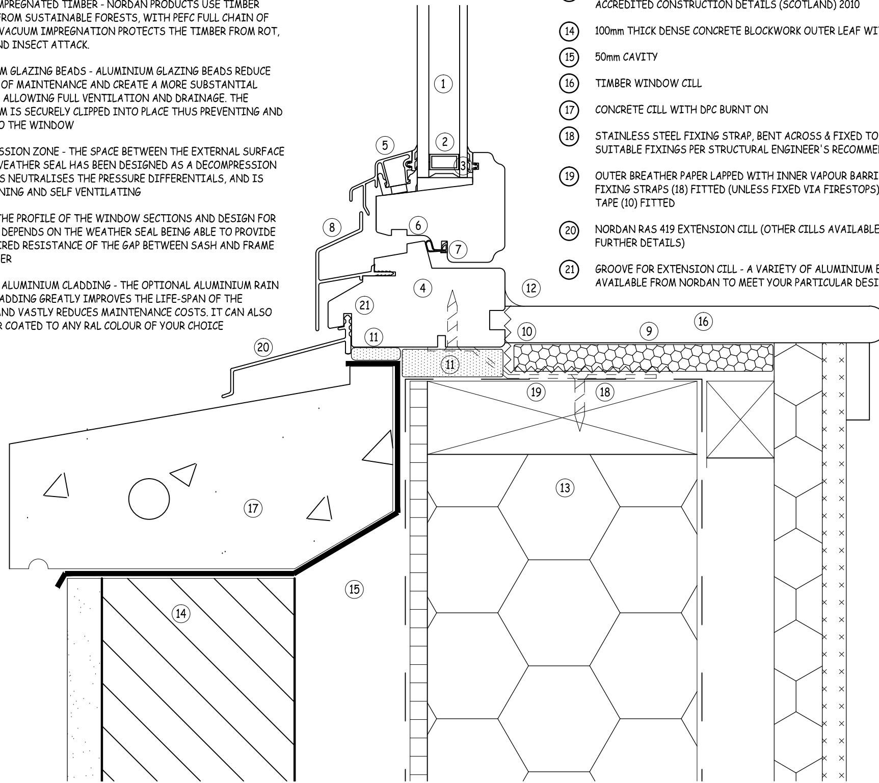
Cill Detail
