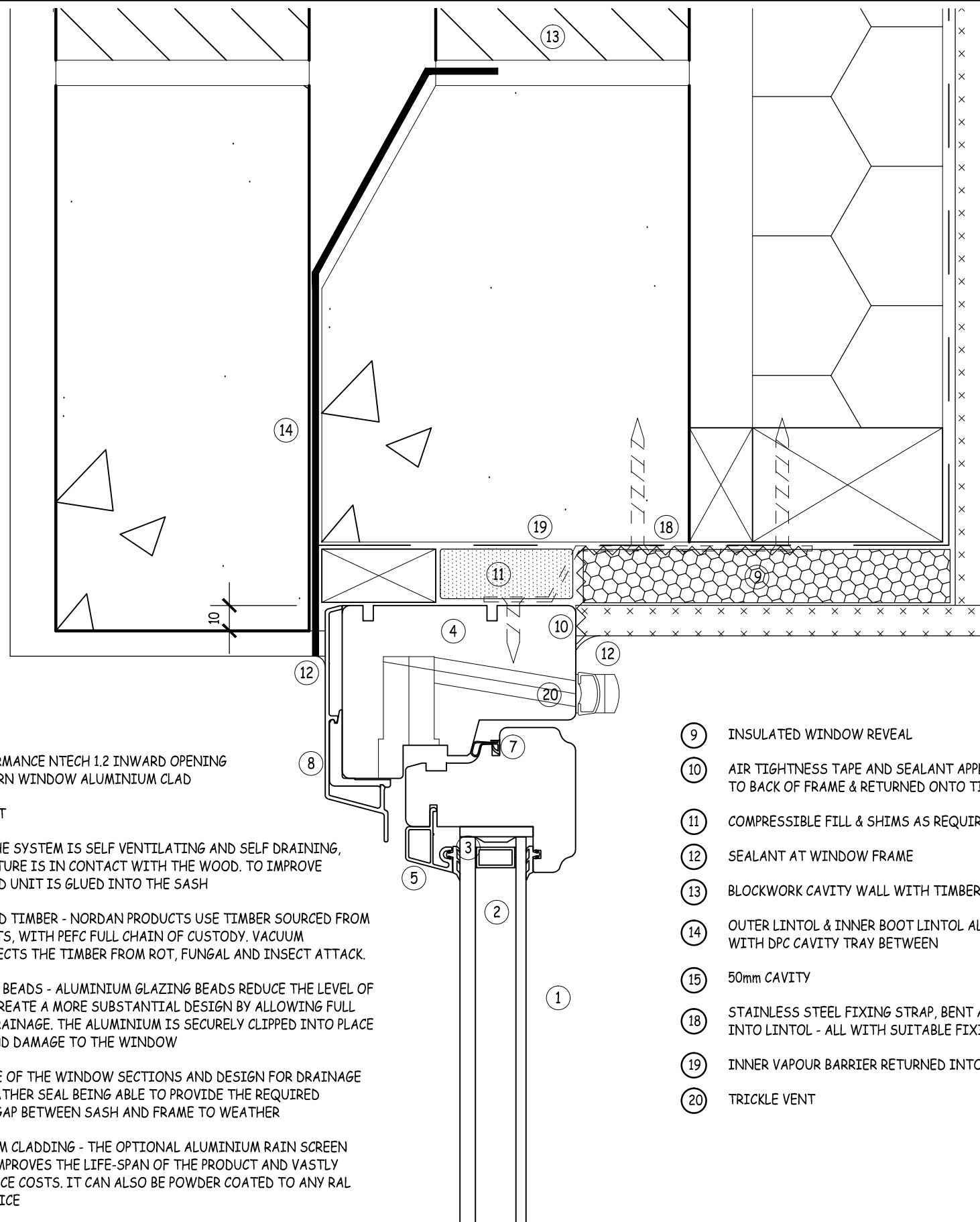
Window Head Detail Scale 1:2 Blockwork Cavity Wall with Framing & Insulation internally
