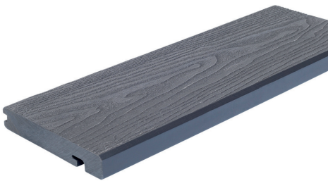
Essential Edge Board Dimensions: 145mm x 24mm x 3600mm
