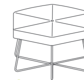
02 POL-WR-BT Pollen buttoned wire base metric (mm) W685 D600 H450 seat 450 imperial (in) W27 D23.5 H17.5 seat 17.5
