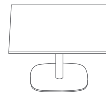
PED-1150-SQ megaped table metric (mm) W1150 D1150 H750 imperial (in) W45.5 D45.5 H29.5
