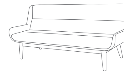
HULO-SF-2000 hush low three seat sofa with timber base metric (mm) W2000 D760 H880 seat 430 imperial (in) W79 D30 H34.5 seat 17
