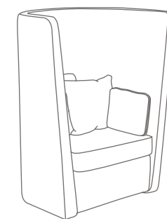
02 BUS-L busby chair left hand metric (mm) W850 D650 H1300 seat 430 imperial (in) W33.5 D25.5 H51 seat 17
