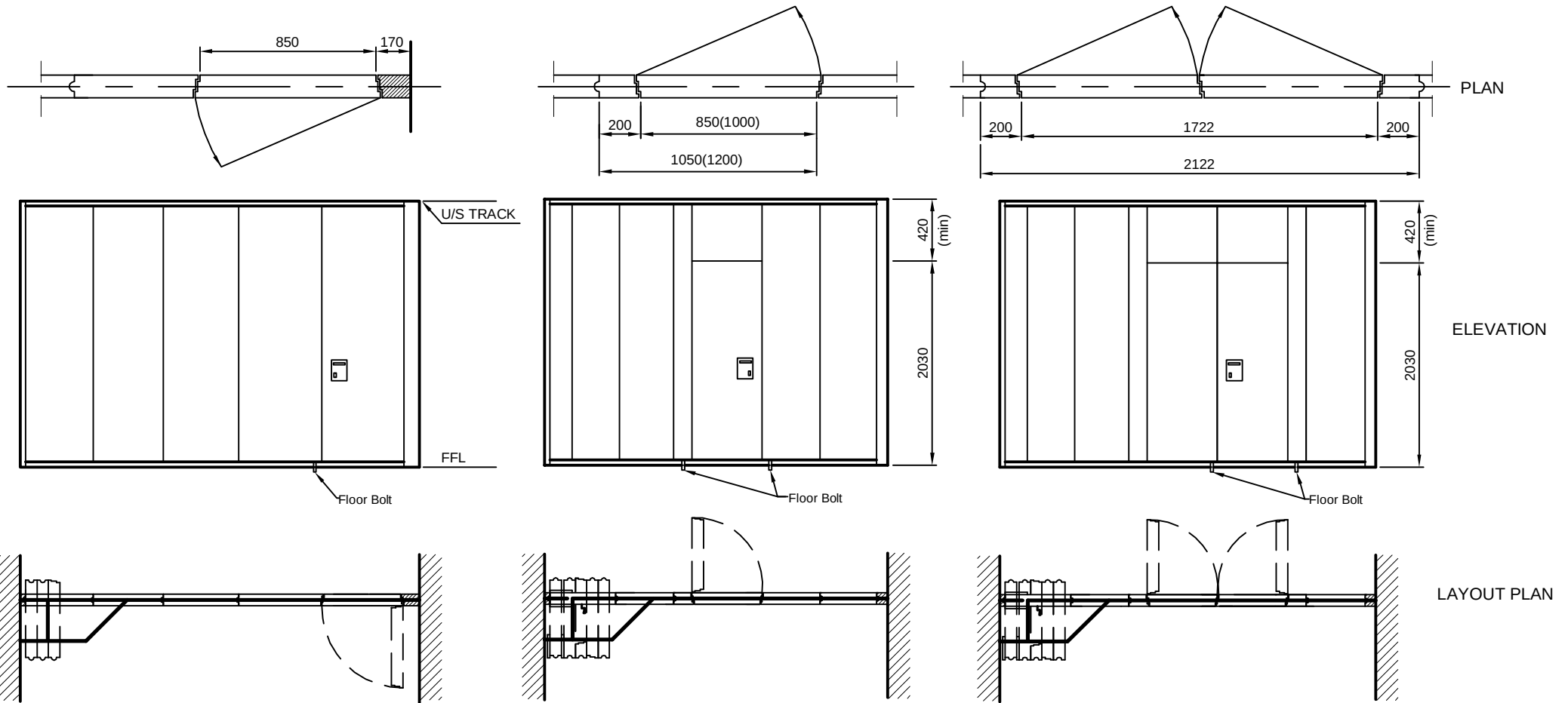
2. Single pass door panel (SE1)
