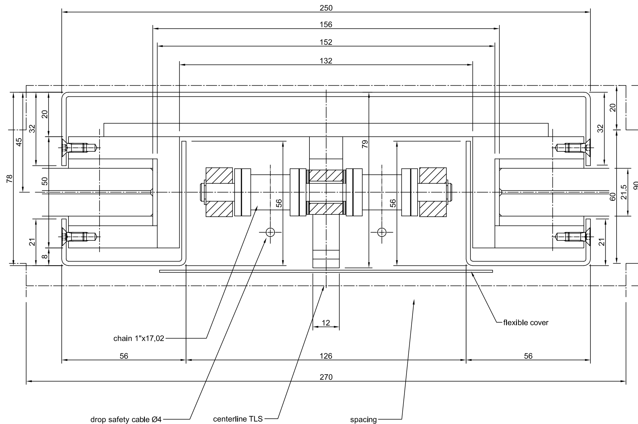
Telescopic railing TLS-U-side Dimensions in mm Scale 1:1
