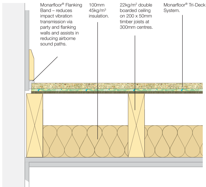
Monarfloor® Tri-Deck over timber joists.
