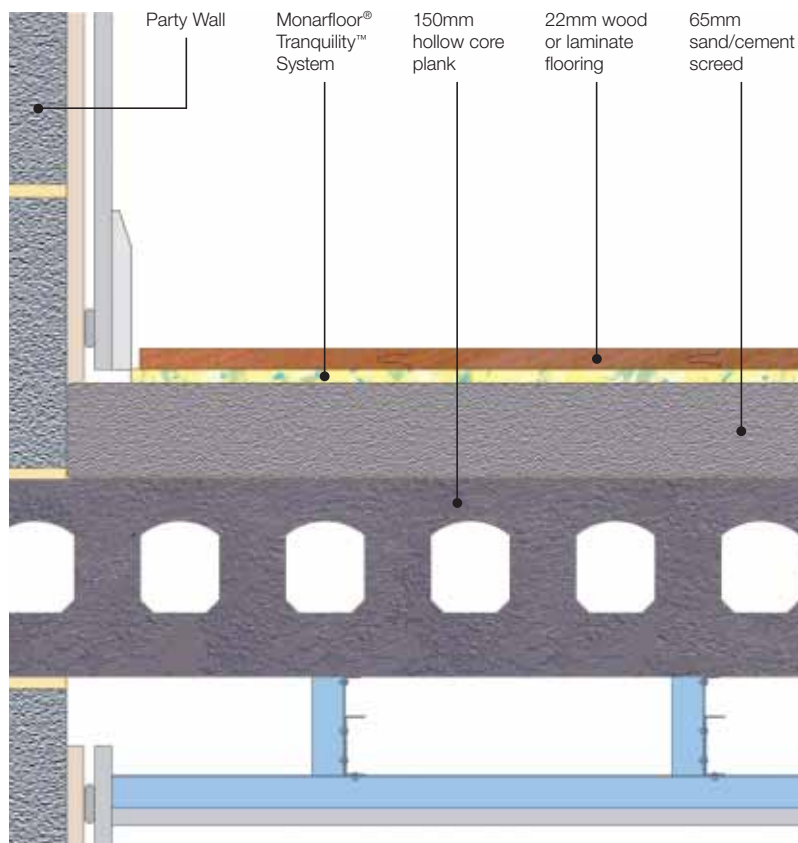
Monarfloor® Tranquility™ over 65mm sand/cement screed on 150mm precast concrete plank (other applications are acceptable please contact Monarfloor Technical Department).
