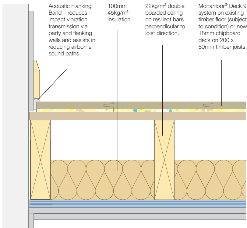
Monarfloor® Deck 9 System on a timber sub-floor with a resilient bar system.
