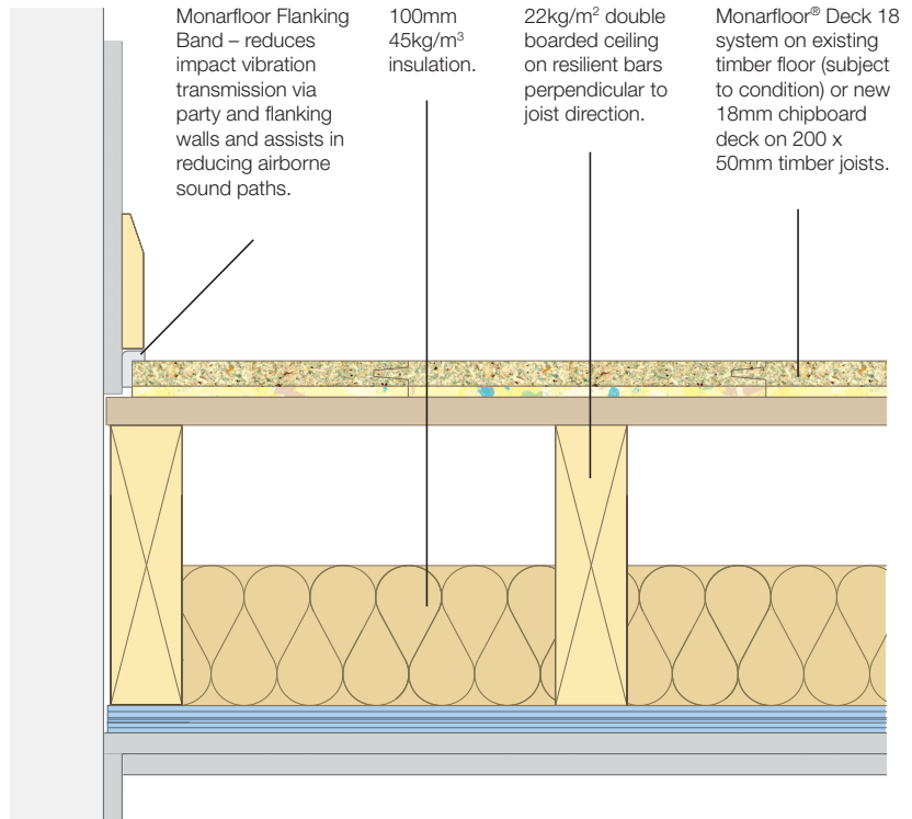
Monarfloor® Deck 18 on a timber floor with a resilient bar system.
