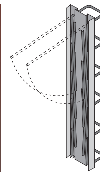
Stabox® S Type B Standard shape case for transverse interlocking
