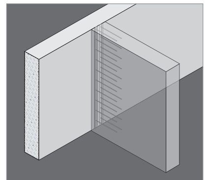
Completely finished wall connection with Stabox rebar connection system.
