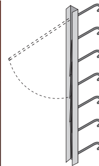
Stabox® Type A or Type H Standard shape case with single row of rebar
