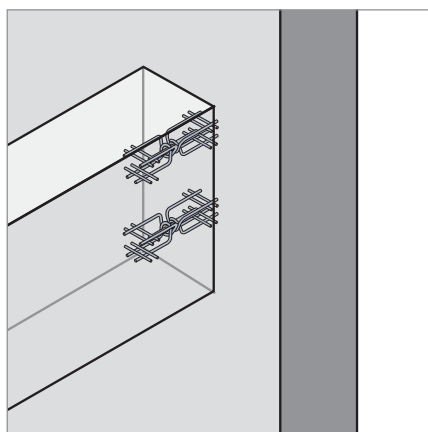
Wall / Girder
