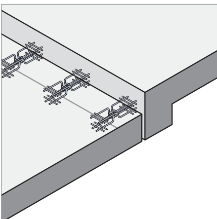
Girder / Slab
