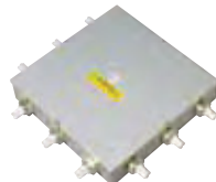
Master distribution unit (MDU) 32Amp rating 260 x 260 x 55mm
