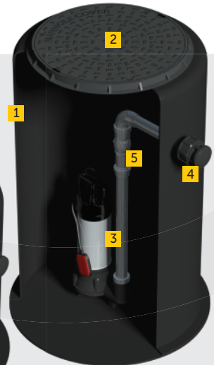
Marsh300F-10 Foul water pump station
