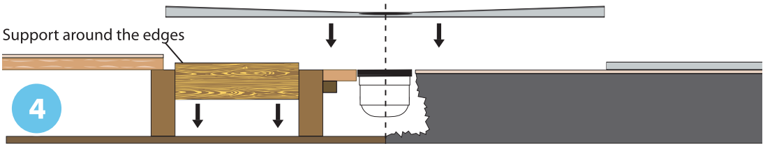
Showerstone directly onto joists
