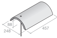
Segmental security ridge tile (code 229)
