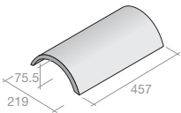
Third round hip tile (code 289)
