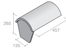
Segmental stop end ridge tile (code 191)
