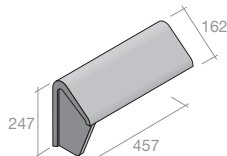
Modern mono block end ridge 15-45° bedded
