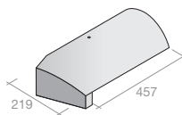
Third round stop end hip
