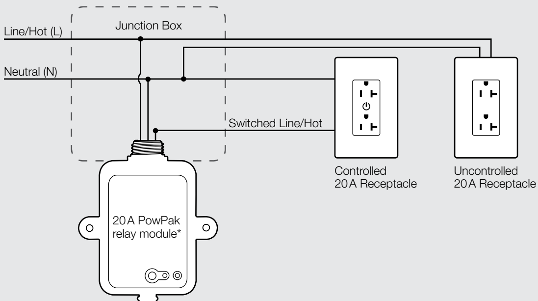
Diagram 2: Duplex Receptacle
