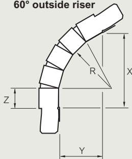
60° outside riser
