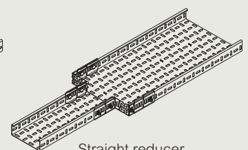
Straight reducer
