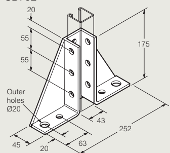
Single channel gusseted bracket SB702
