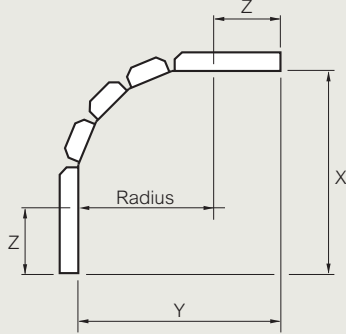
90° outside riser
