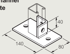
Double channel base plate SB705
