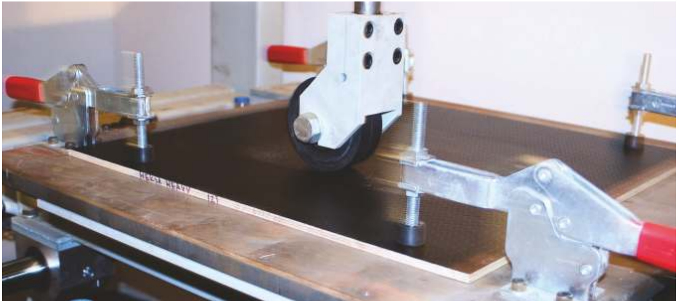
Figure 3.3. Determination of the effect of loaded heavy duty castors
