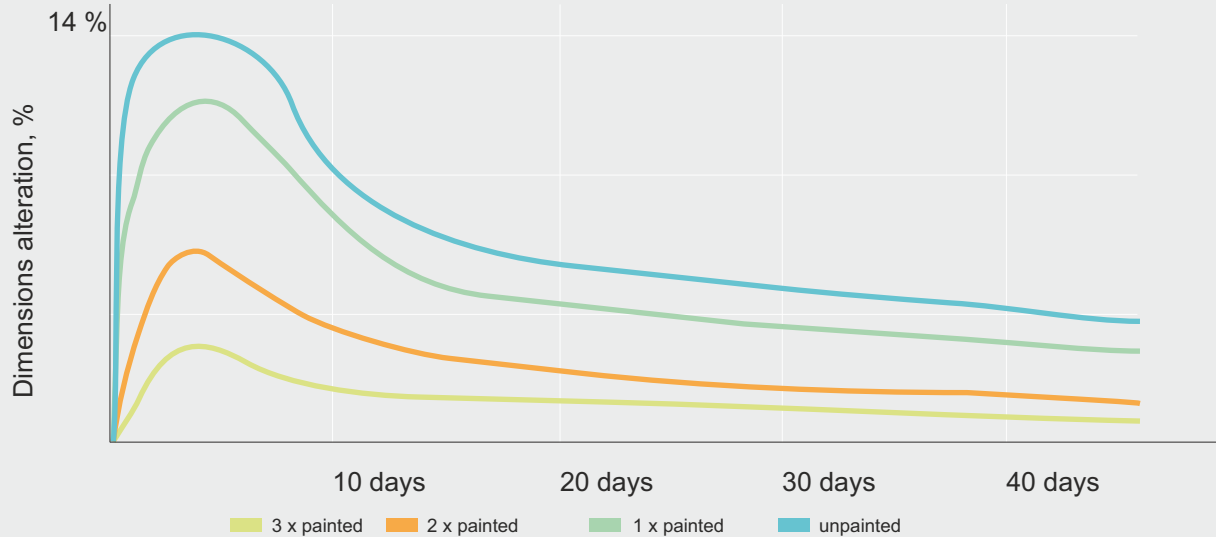
Figure 6.8. Dimension alteration of 18 mm plywood panel overlaid with phenol film, in %, 2 cm from the edge, after immersion in water for 48 hours and drying
