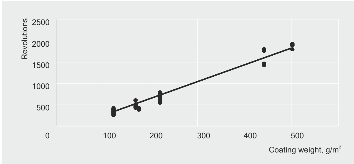
Figure 3.2. Wear resistance of Riga Form plywood
