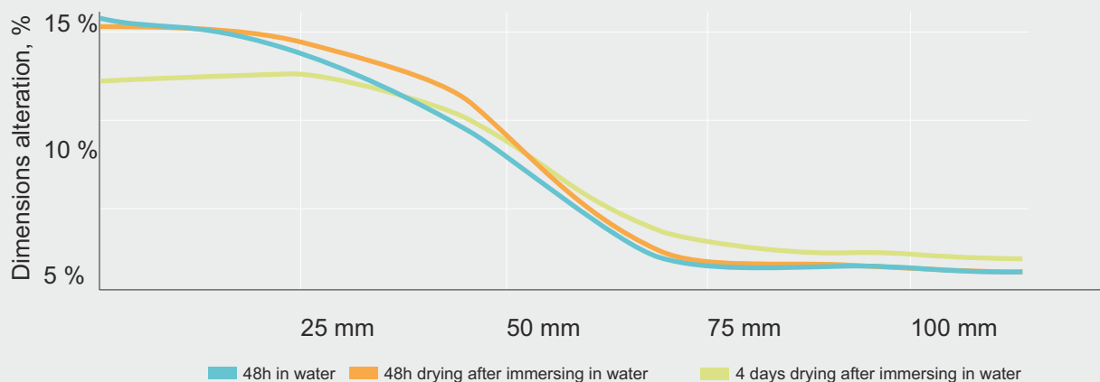
Figure 6.9. Dimension alteration
