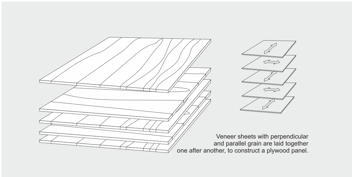
Figure 2.4. Plywood lay-up scheme
