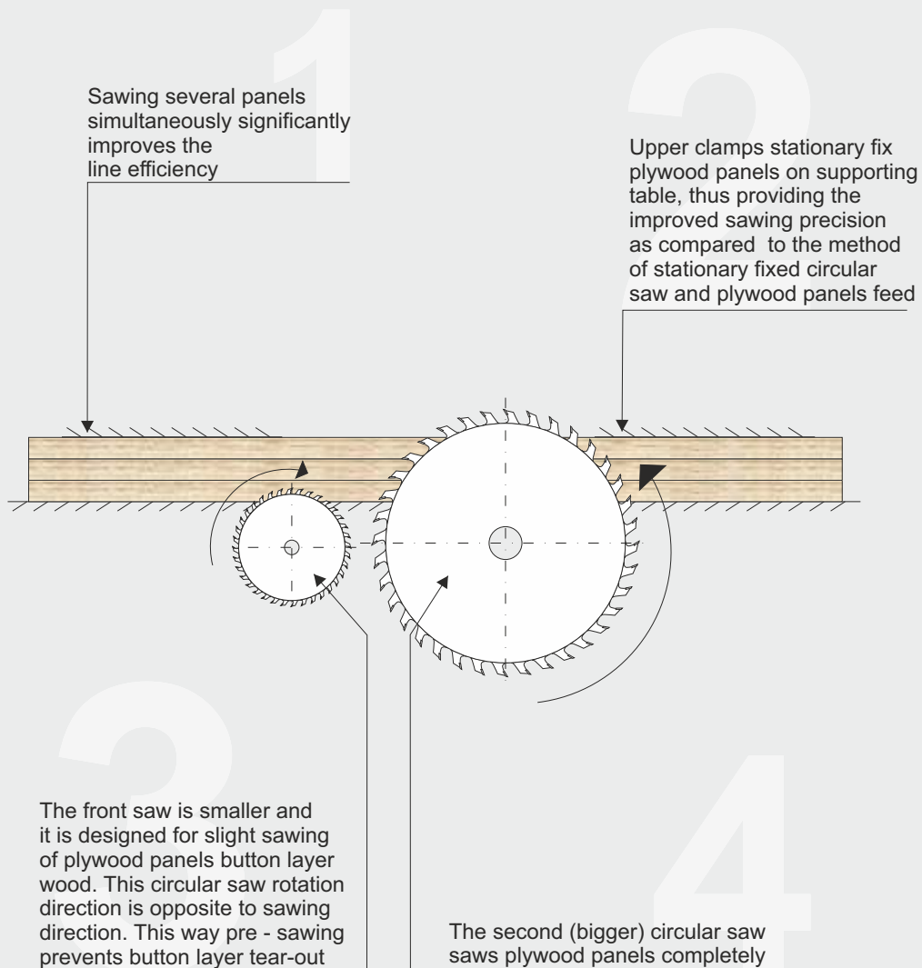
Figure 6.6. Cutting scheme
