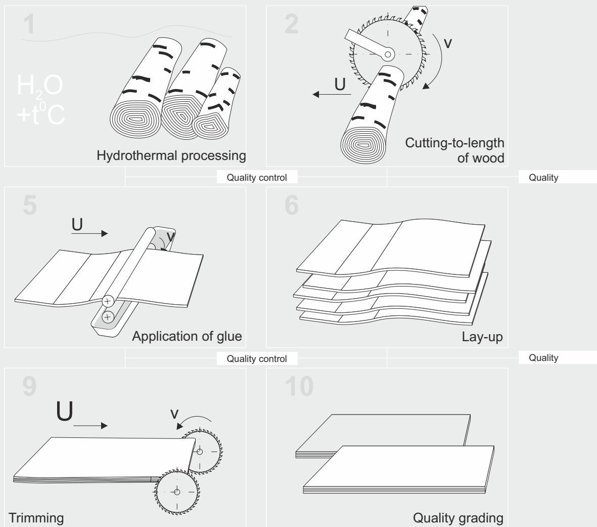
Figure 2.1. Plywood production diagram
