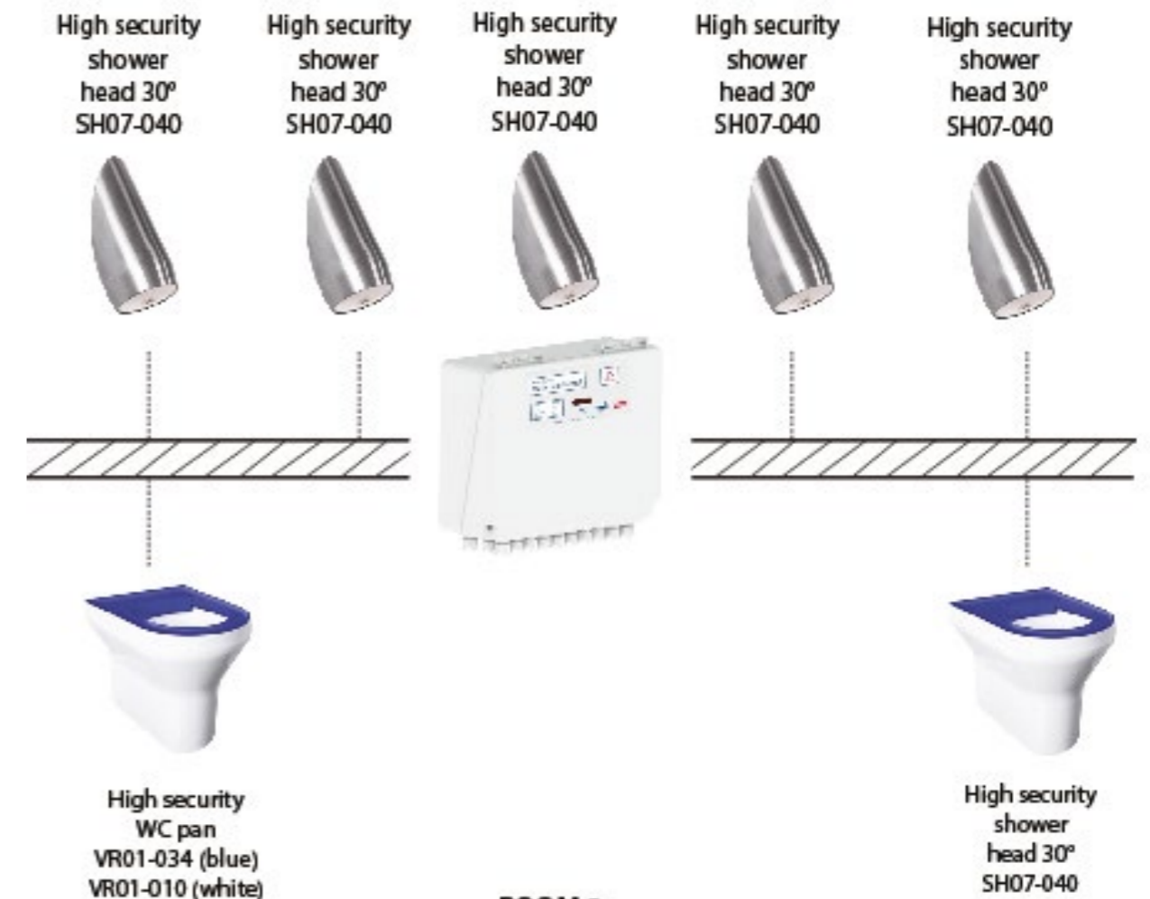
ROOM 2
