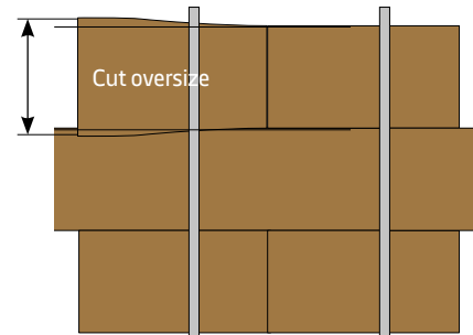
Brick tie channel
