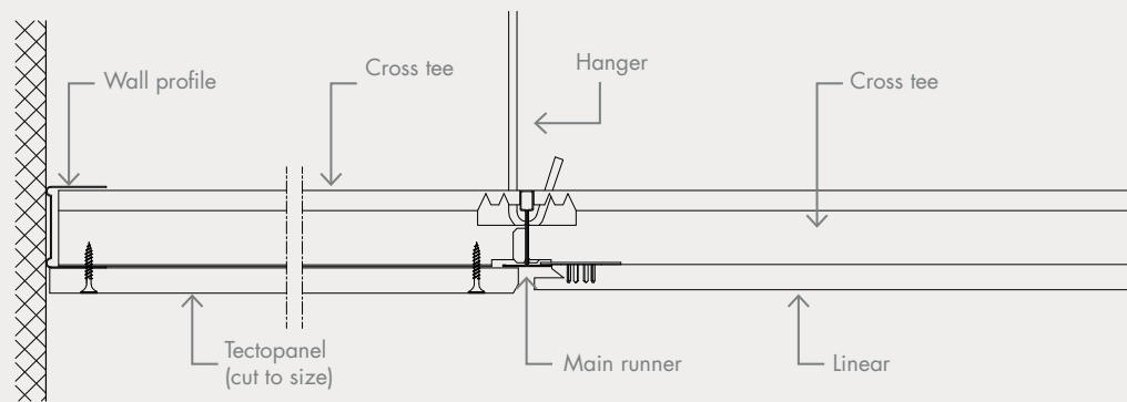
Linear in grid system S24 with fixed frieze
