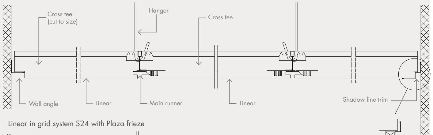
Linear in grid system S24 direct to wall
