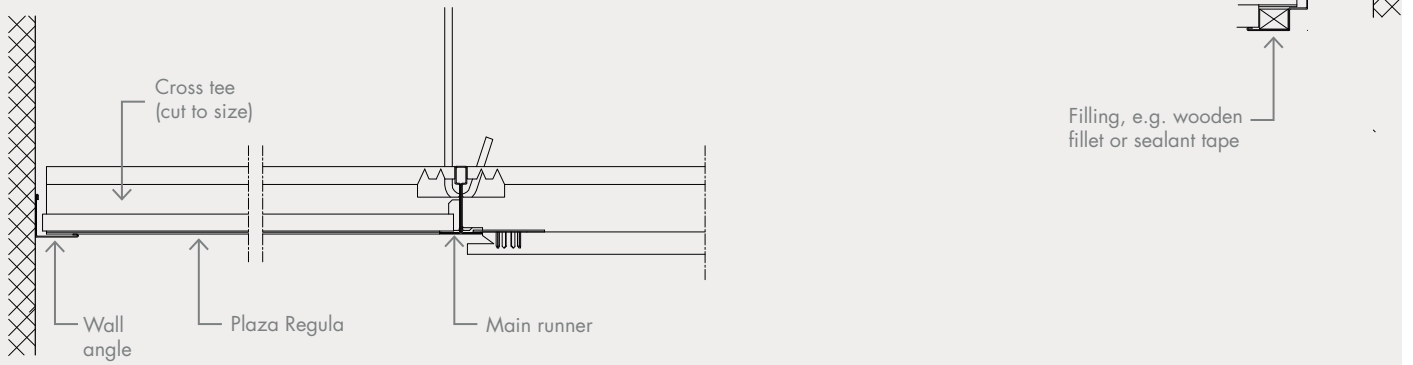
Linear in grid system S24 with Plaza frieze
