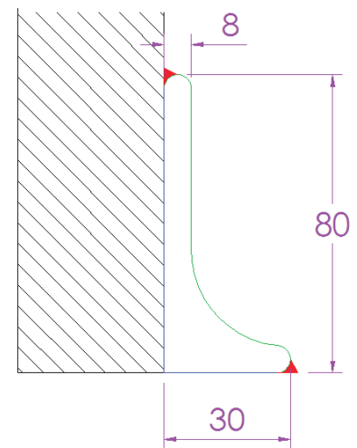
PolySto PV8F Skirting installation illustration
