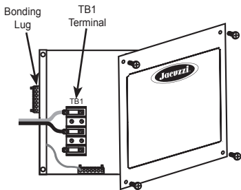
Figure 15 3-wire, 120 VAC Connection for Models J-210, J-315, and J-325
