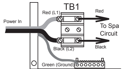
Figure 9 3-Wire, 240 VAC Connection (Hard-wired connections only)
