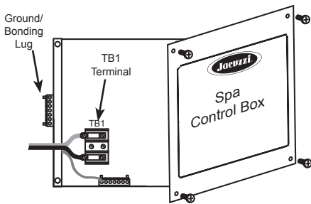
Figure 8 The Control Box for 3-wire, 240 VAC connection. (The location of the TB1 terminal may vary between models.)
