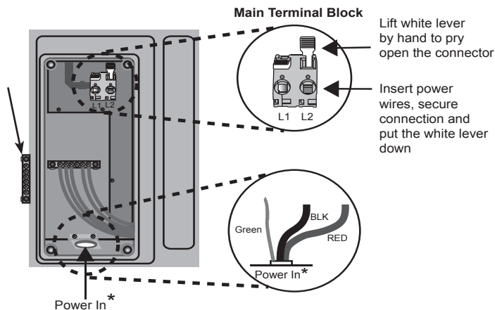
Figure 4 Control Box for 3-Wire, 240 VAC Connection for Models J-415, J-425, J-465, J-470, J-480 and J-495 (For hard-wired connections only)
