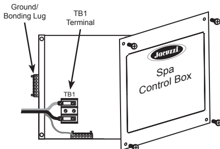
Figure 11 The Control Box for 3-wire, 240 VAC connection
