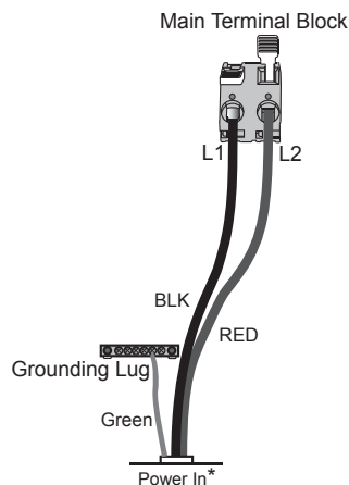
Figure 5 3-Wire, 240 VAC Connection for Models J-415, J-425, J-465, J-470, J-480 and J-495 (For hard-wired connections only)
