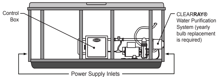
Figure 14 The Control Box for Models J-210, J-315, and J-325
