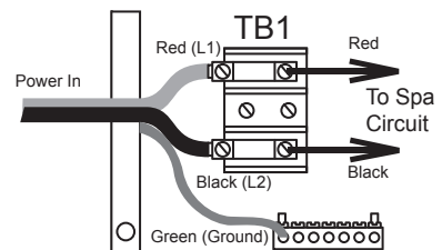
Figure 12 3-Wire, 240 VAC Connection for Models J-235, J-245, J-275, J-280, J-335, J-345, J-355, J-365, J-375, J-385 (For hard-wired connections only)
