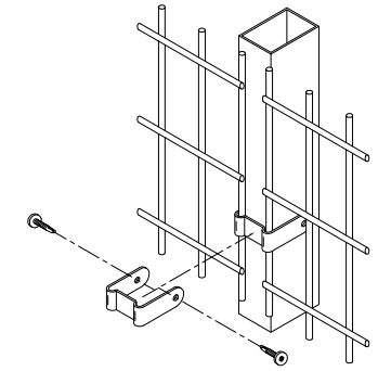
FIXING BRACKET DETAIL
