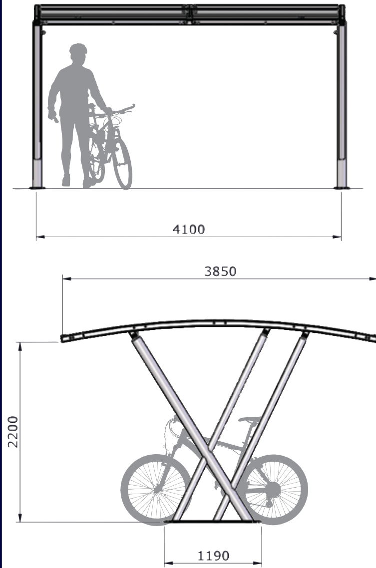
DOUBLE BANBURY DIMENSIONS(mm)3850W X 2200H X4100L
