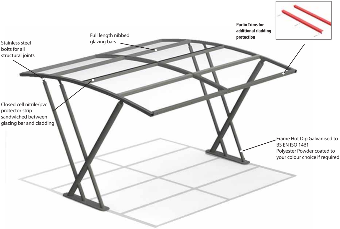
DOUBLE BANBURY DIMENSIONS(mm)3850W X 2200H X4100L
