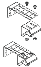
Intermediate Bracket with 2" Extension Bracket
