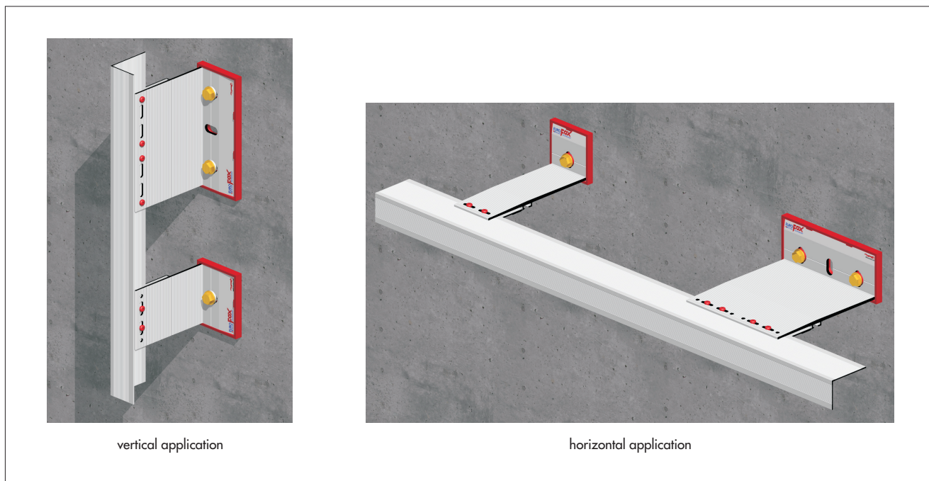
Figure 3 Typical rail/bracket arrangement
