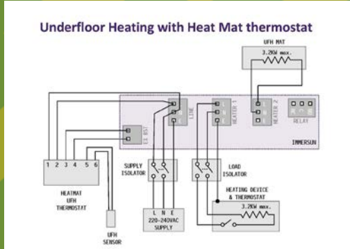
Example wiring diagram connecting Heat MatPV with an ImmerSun unit.
