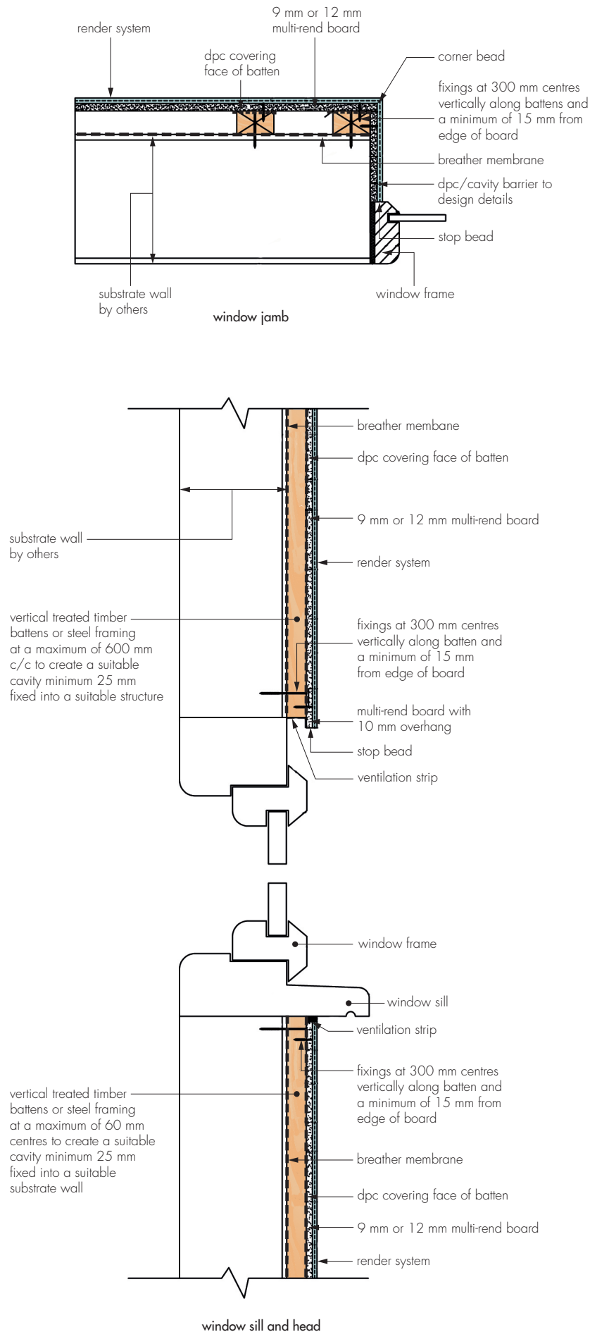
Figure 2 Opening details — Timber Frame
