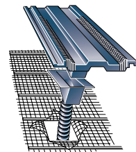
HD RSPA Tile vent adapter kit for use with HD TV10/6 and 10/8 range of ventilators.
