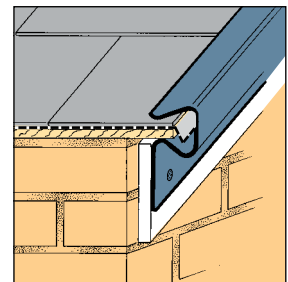
Sprocket Joint Fig 2
