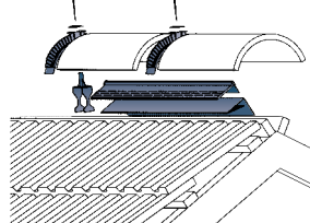
DFR3 DRY FIX RIDGE/VENTILATION SYSTEM
