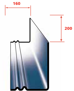
HDL SCSS Conti-Soaker™.
