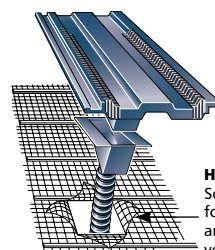
DFR3 DRY FIX RIDGE/VENTILATION SYSTEM
