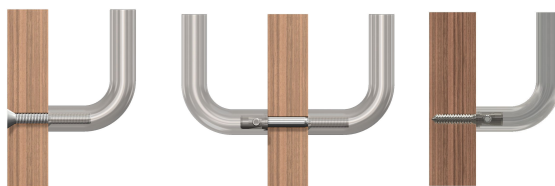
Bolt through
