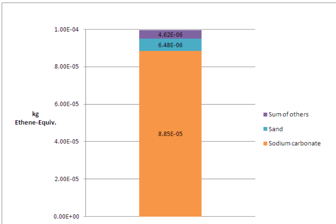
Figure 19: POCP from batch materials production per 1 kg float glass, cradle-to-gate
