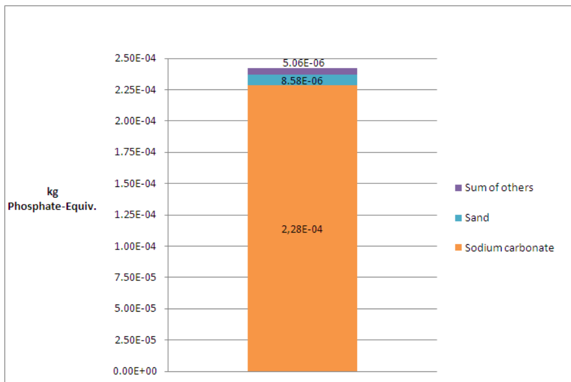
Figure 11: EP from batch materials production per 1 kg float glass, cradle-to-gate
