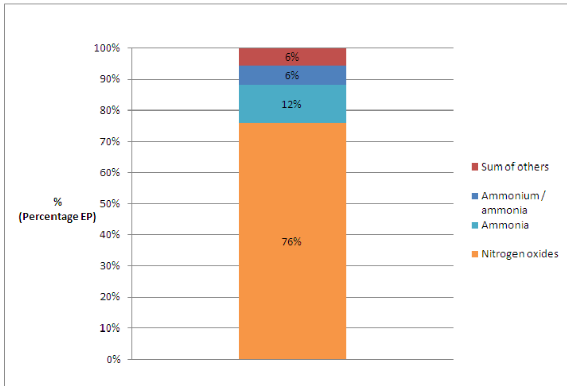
Figure 10: Total EP main contributing emissions per 1 kg float glass, cradle-to-gate
