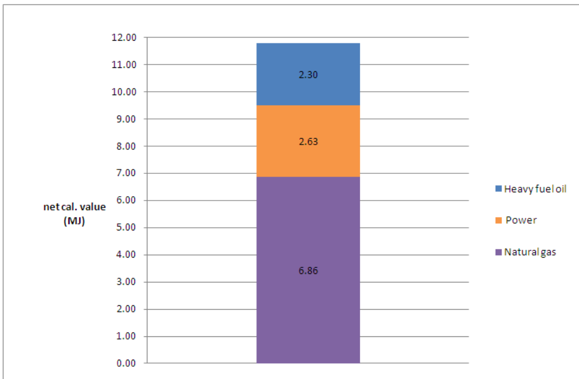
Figure 8: PED from energy sources per 1 kg float glass, cradle-to-gate
