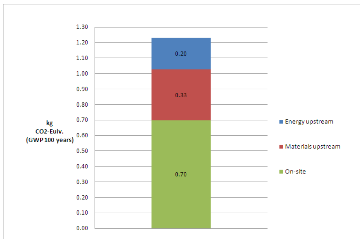
Figure 2: Total GWP for 1 kg float glass, cradle-to-gate
