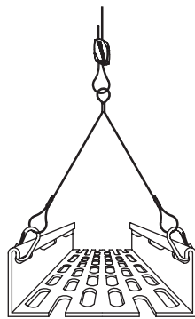
Y-Fit accessory with Link hook on cable tray
