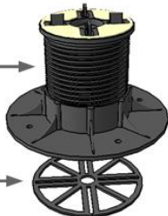
PAVING SUPPORT ILLUSTRATIVE CUTTING GUIDE.
