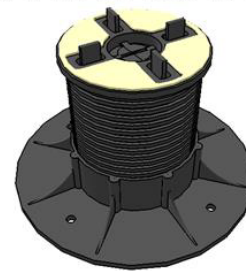
Condition 03 (4 Tile junction)
