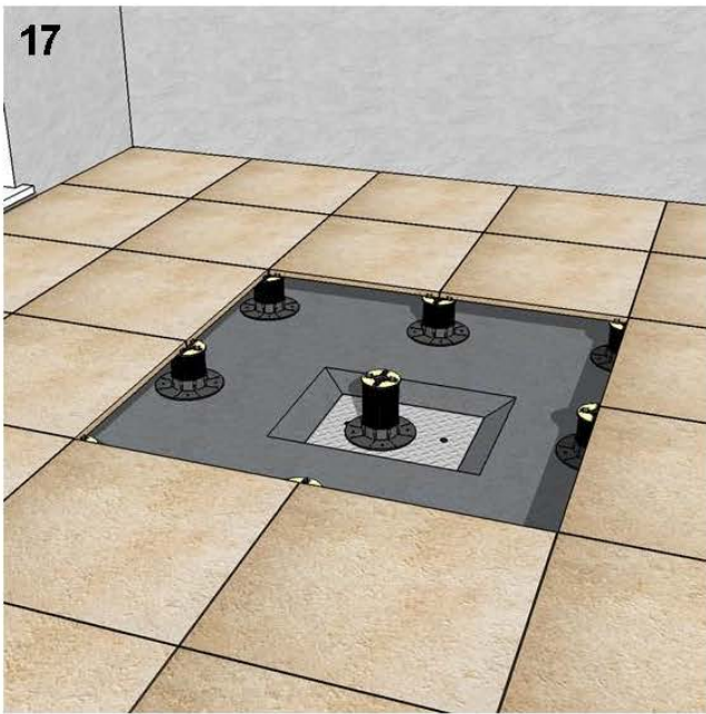
17 - For recesses, recessed manholes/drains or level changes, you may require longer NM pedestals which should be set out and installed in exactly the same manner as all other pedestals. See our full range of accessories so that you select the appropriate pedestals to suit your application.
