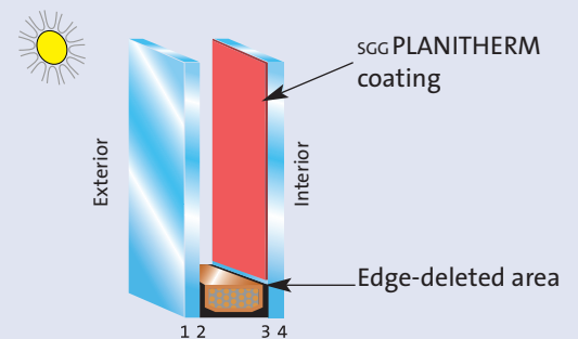
Insulating glass unit with SGG PLANITHERM (coating on face 3)
