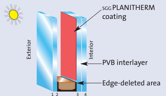
Insulating glass unit with laminated SGG PLANITHERM (coating on face 3)
