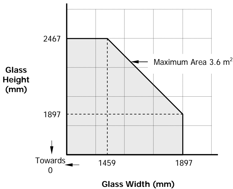
Figure 11. Maximum Permitted Glass Dimensions
