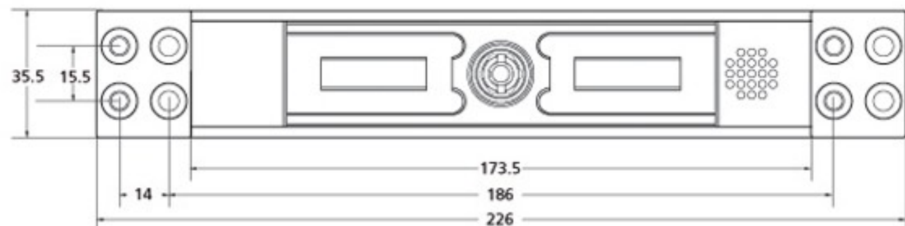
Magnet
