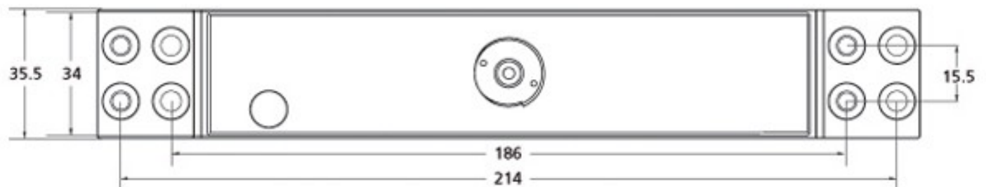
Magnet
