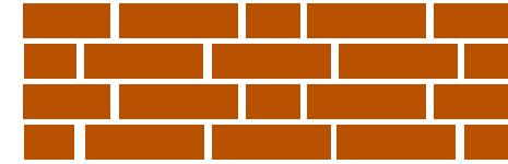
Flemish Garden Bond
