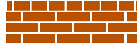
English Garden Wall Bond
