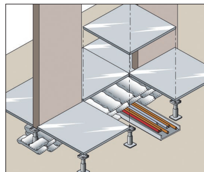
Firewise Intumescent Pillows forming cavity barrier underneath raised access floor
