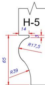
Trykvent
