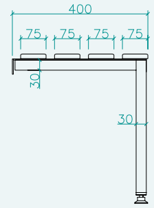
SGL Slats (Section View)
