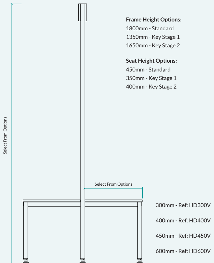
Double Island Bench Frame
