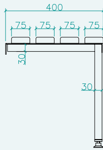
Ash Slats (Section View)
