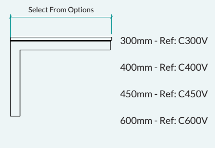
Cantilevered Wall Bench Frame
