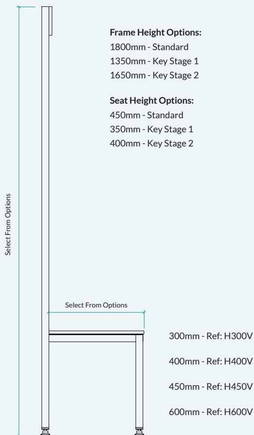
Single Island Bench Frame
