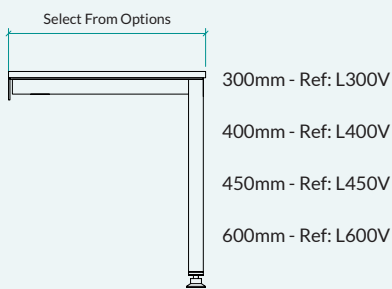
Single Wall Bench Frame
