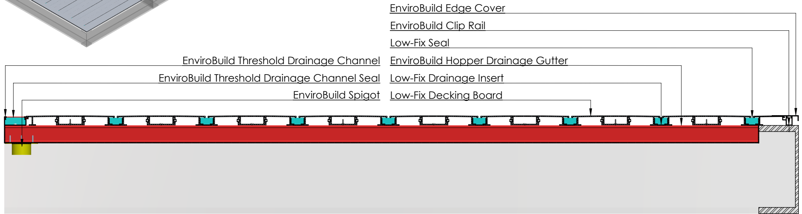
SECTION B-B
